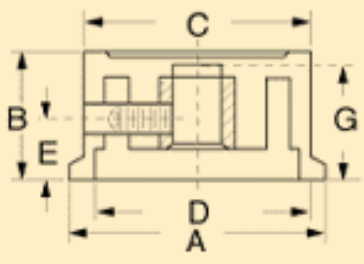
Brass Bushing w/ Set Screw
